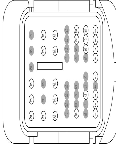
FEMALE Harness: 14631
